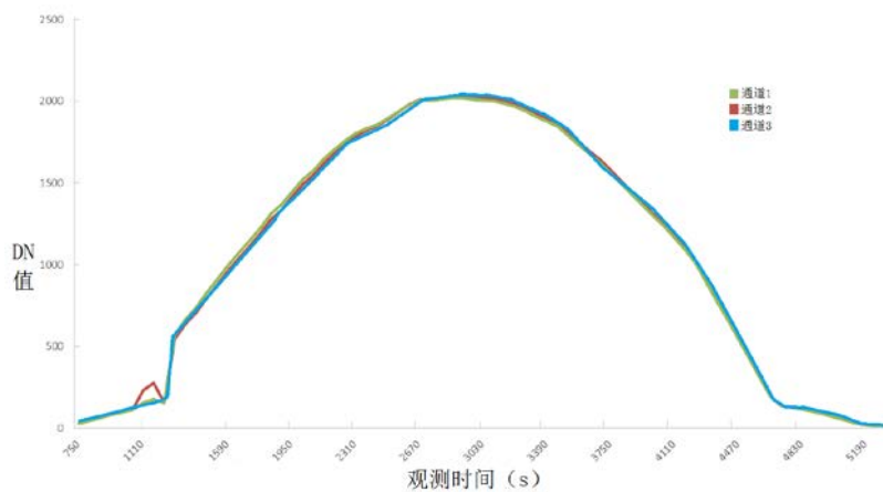
Fig. 9. Time-variation Analysis of the Light Intensity Measurement
