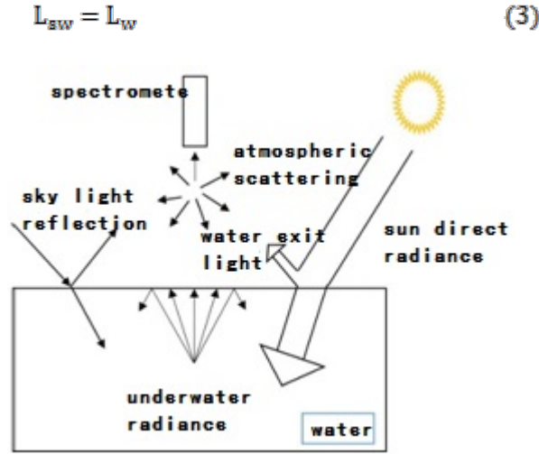
Fig. 1. Signal Composition of the Water Surface
