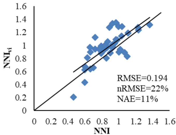
Fig. 2. Comparison of NNI_{vi} and NNI
