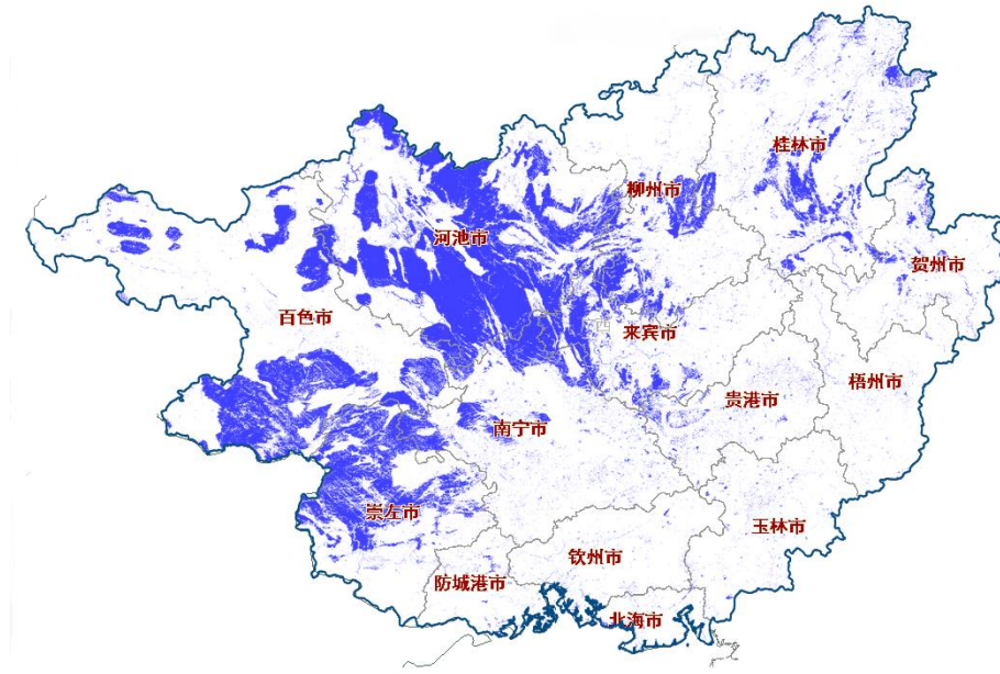
Fig. 1. Karst rocky areas of Guangxi Province
