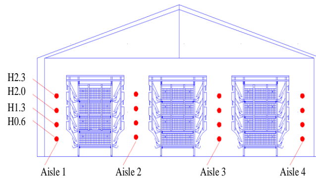
(b) The diagram of transverse henhouse aisle sampling points
