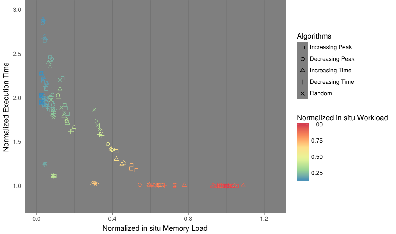
Figure 7: Evaluation of in situ memory and workload parameters in algorithm performance for asynchronous scenario.
