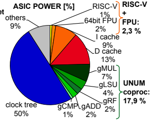
Figure 9: Chip power distribution
