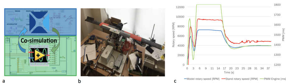
Fig. 10. Hardware-in-the-Loop scheme (a), HiL test-bench (b), HiL test-model comparison results c
