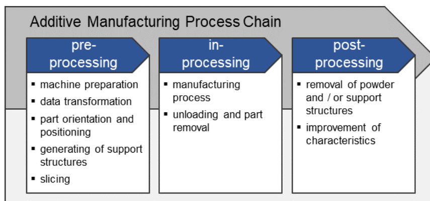
Fig. 1. The AM process chain with the three phases pre-, in- and post-processing
