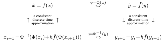
Fig. 1. The scheme of the consistent implicit discretization of \dot{x} = f(x)
