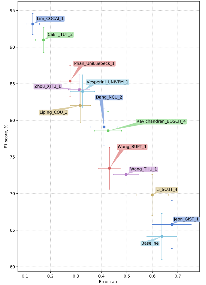
Fig. 3. Scatter plot of submitted systems for Task 2 accompanied by the 95% confidence intervals. Systems were ranked by ER (the smaller the better).
