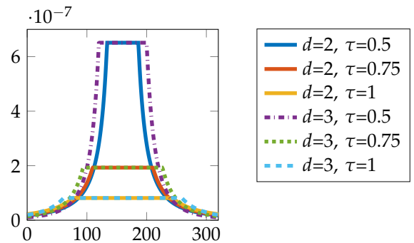
Fig. 3. The 6 tested densities \nu for N = 320 .
