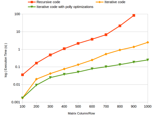
Figure 3. Performance results with the matrix product
