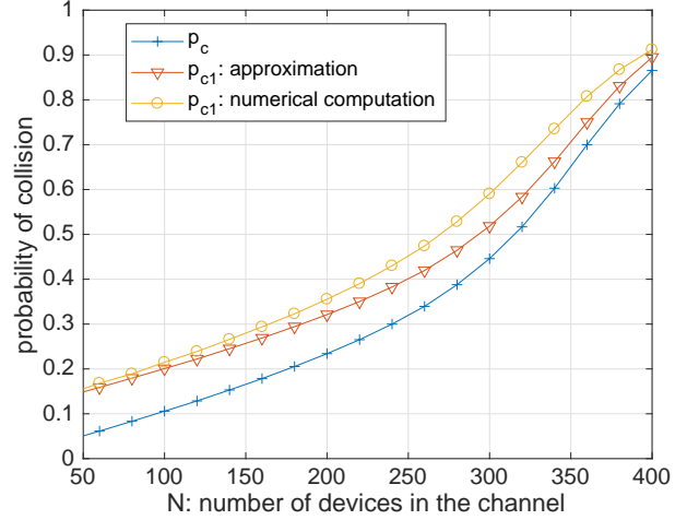
Fig. 2. Our proposed approximation for the probability of collision at the second transmission. It is more precise for smaller values of N .
