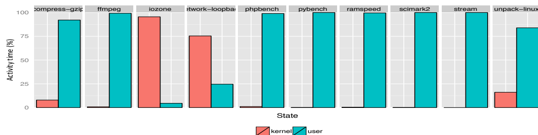
Figure 7. User vs kernel time (x86 desktop machine)
