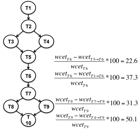
Fig. 9 The reuse pattern found in the Lattice benchmark
