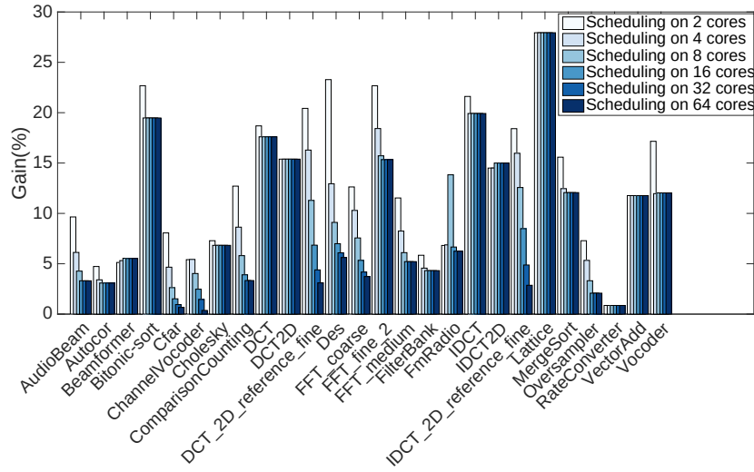
Fig. 10 Impact of the number of cores on the gain of CLS against NCLS
