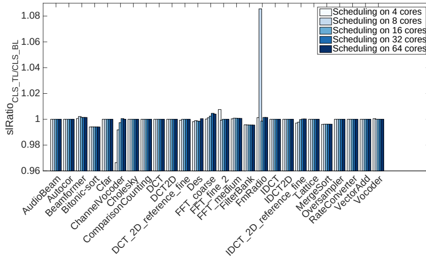
Fig. 11 Comparison of schedule lengths for CLS.TL and CLS.BL
