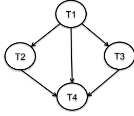
Fig. 12 The schedule graph constructed based on the scheduling information in the adapted cache-conscious schedule as depicted in Figure 6
