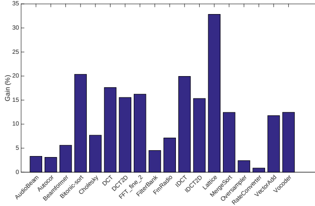
Fig. 7 Gain of CILP as compared to NCILP ( gain = \frac{sl_{NCILP} - sl_{CILP}}{sl_{NCILP}} * 100 ) on a 16 cores system
