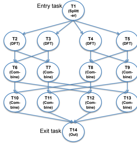
Fig. 2 Task graph of a parallel version of a 8-input Fast Fourier Transform (FFT) application [4]
