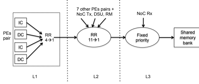
Fig. 3 SMEM memory request flow [13]
