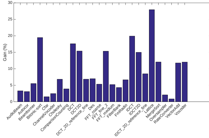
Fig. 8 Gain of CLS as compared to NCLS ( gain = \frac{sl_{NCLS} - sl_{CLS}}{sl_{NCLS}} * 100 ) on a 16 cores system
