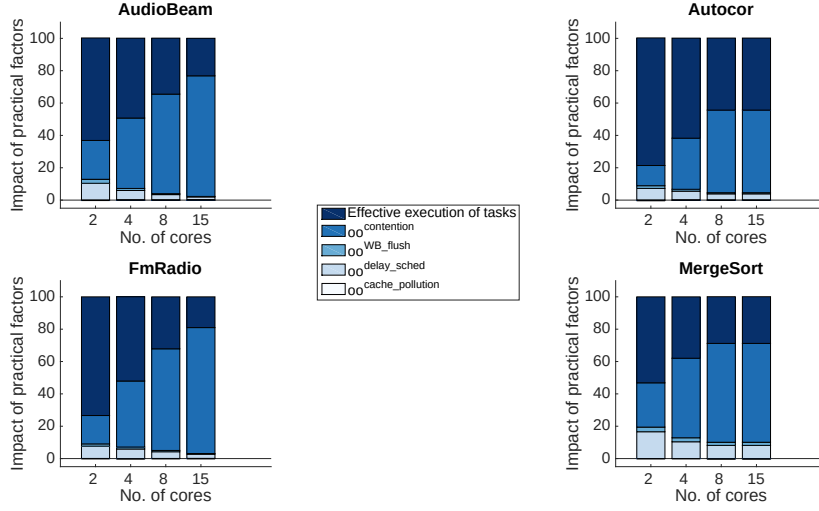
Fig. 13 The impact of different implementation factors on the adapted cache-conscious schedules
