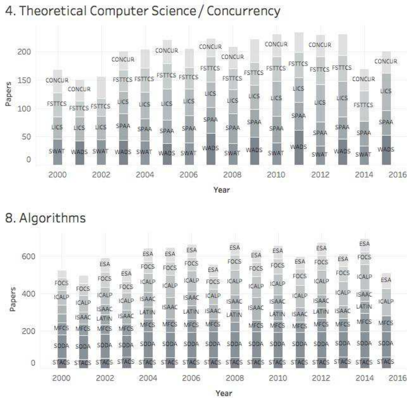
Fig. 5: Comparison of the publication growth rate per year of TCS/C and ALGO.
