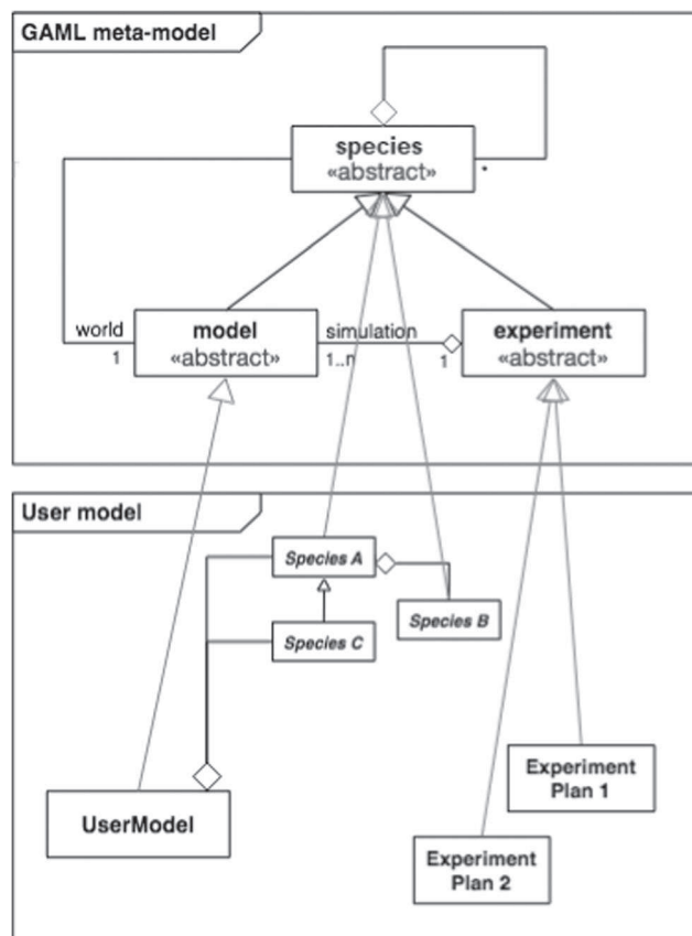
Fig. 2 Main concepts behind GAML
