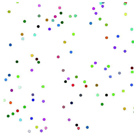
Fig. 3 a GAML code of the simpleModel : this model creates 100 simple agents displayed by a circle with a random color; at each simulation step, these agents move randomly; b snapshot of the resulting simulation
