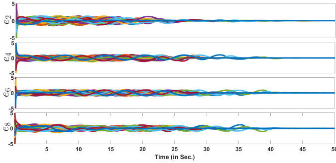
Figure 2. Evolution of errors e_{2i} = x_{2i} - x_{2(i+1)} , i = \overline{1, 4} with randomly selected initial conditions for 50 simulations run.
