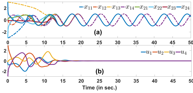
Figure 1. The results of simulation of (11), (26) for N = 4 . a) Evolution of the oscillator states; Bottom) Control signals.
