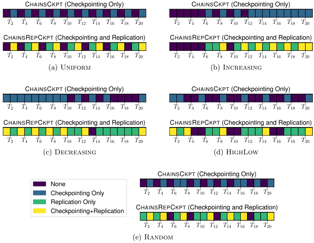
Figure 2: Optimal solutions obtained with the CHAINSCkPT algorithm (top) and the CHAINSREPCkPT algorithm (bottom) for the five work distributions.
