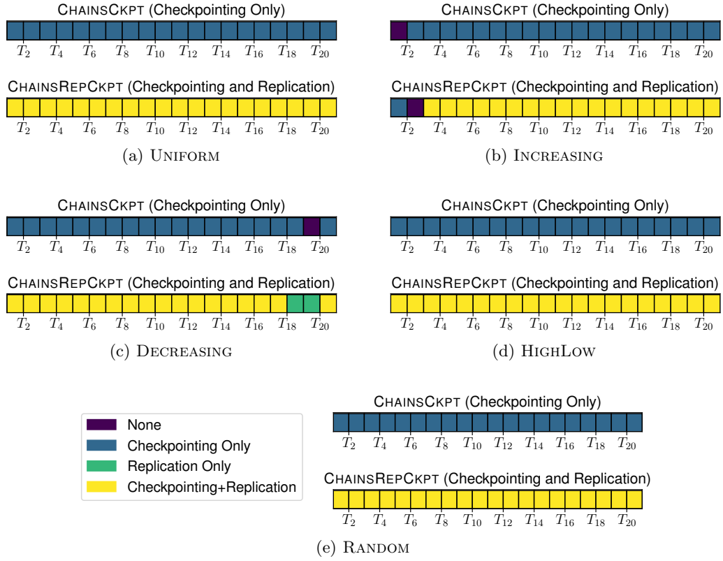
Figure 8: Optimal solutions obtained with the CHAINSCkPT algorithm (top) and the CHAINSREPCkPT algorithm (bottom) for the five work distributions.
