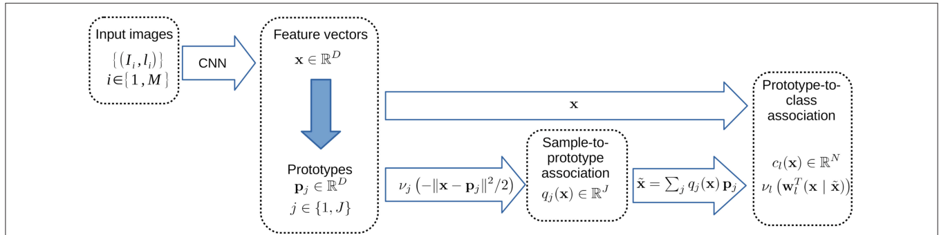
FIGURE 1 | The three layer model. The input data is fed to a convolution neural network, transforming the original image into a set of feature vectors. Then the information in this high dimensional feature space is summarized via a set of prototypes, in order to understand the landscape. Finally, the relation between a given data point and the label to infer is calculated through their proximity to the prototypes.
