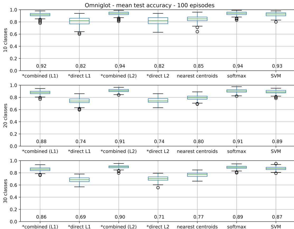
FIGURE 8 | Box plots for test accuracies over 100 episodes. Boxes extend between 1st and 3rd quartiles ( IQR ), with median value noted at the bottom and marked by a green line. Bars mark a range of \pm 1.5 IQR from quartiles, with outliers as circles. Our models are marked with a *.
