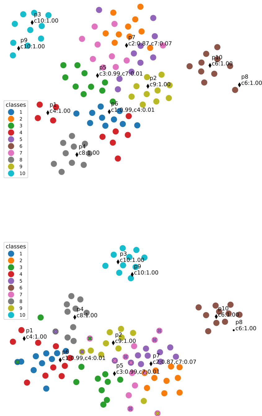
FIGURE 7 | T-SNE visualizations of dataset points (as Inception v3 features) together with learned prototypes, indicated by black markers. Each class is identified by color, and the predicted class for each prototype is annotated. Misclassified points are over-marked by an “x” of the predicted class color. (Top) Visualization of the training set; (Bottom) Visualization of the test set.
