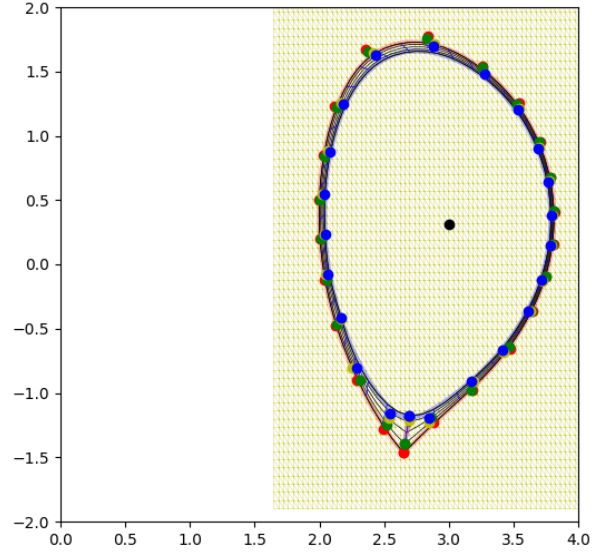
Figure 28: One-element surface containing an-x-point
