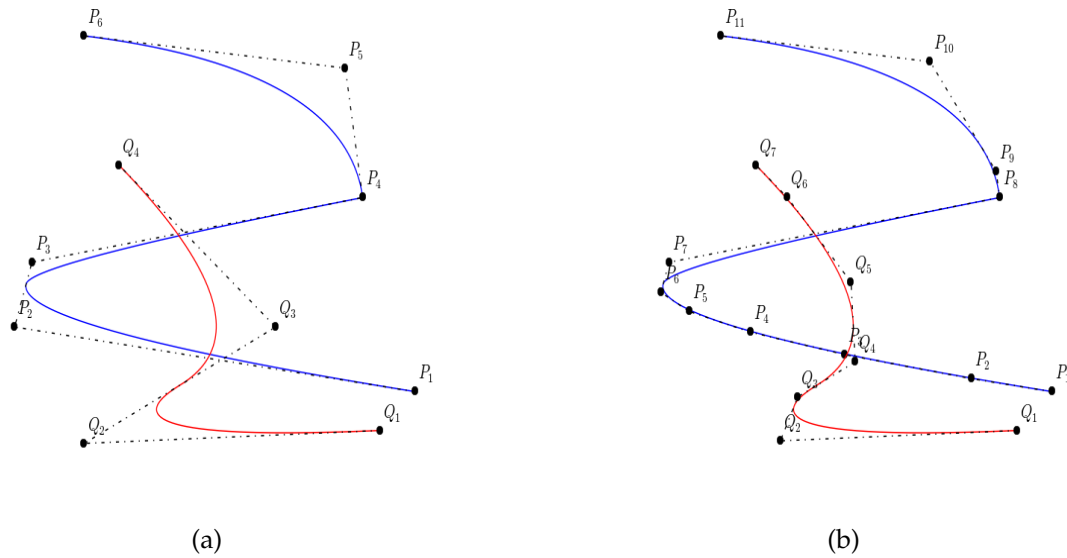
Figure 6: (a) Two quadratic B-spline curves and their control polygons. The knot vector for the blue curve is \{000, \frac{1}{2}, \frac{3}{4}, \frac{3}{4}, 111\} while for the red curve it is \{000, \frac{1}{2}, 111\} . (b) Curves and their control polygons after inserting the knots \{0.1, 0.2, 0.3, 0.4, 0.8\} in the blue curve and \{0.4, 0.7, 0.9\} in the red curve. Intersections of the two control polygons approximate the intersection of the two curves.
