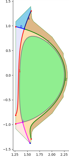
Figure 22: A disconnected double null in the DIII-D tokamak
