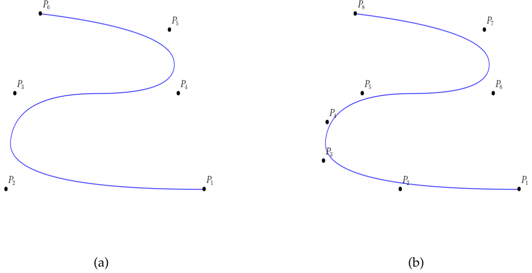
Figure 5: (a) A quadratic B-spline curve and its control points. The knot vector is T = \{000, \frac{1}{4}, \frac{1}{2}, \frac{3}{4}, 111\} . (b) The curve after a h-refinement by inserting the knots \{0.15, 0.35\} while the degree is kept equal to 2.
