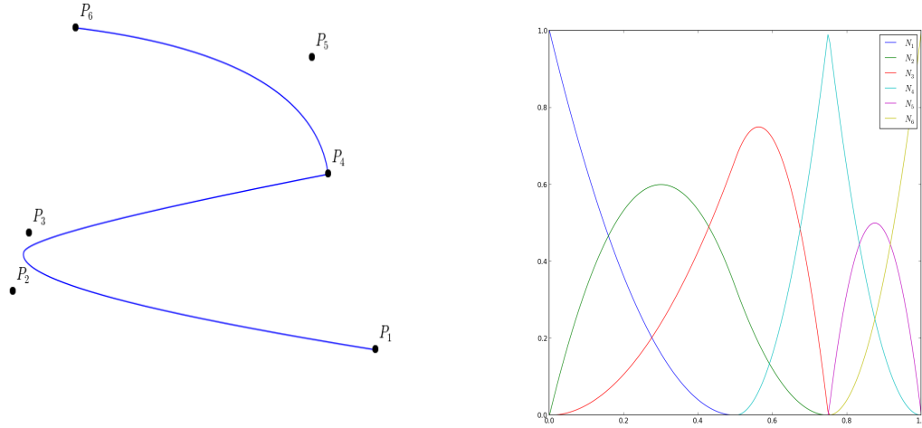
Figure 4: (left) A quadratic B-Spline curve and its control points (the knot vector is \{000 \frac{1}{2} \frac{3}{4} \frac{3}{4} 111\} ), (right) the corresponding B-Splines.
