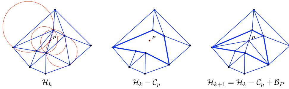
Figure 18: Illustration of the incremental Delaunay insertion of a point in a mesh.
