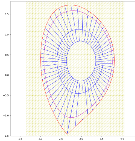
Figure 30: \mathcal{G}^1 regular grid inside the Separatrix.
