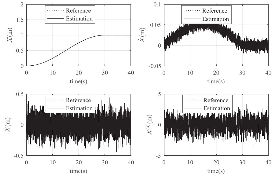
Figure 9. Simulation results of the channel X with measurement noise
