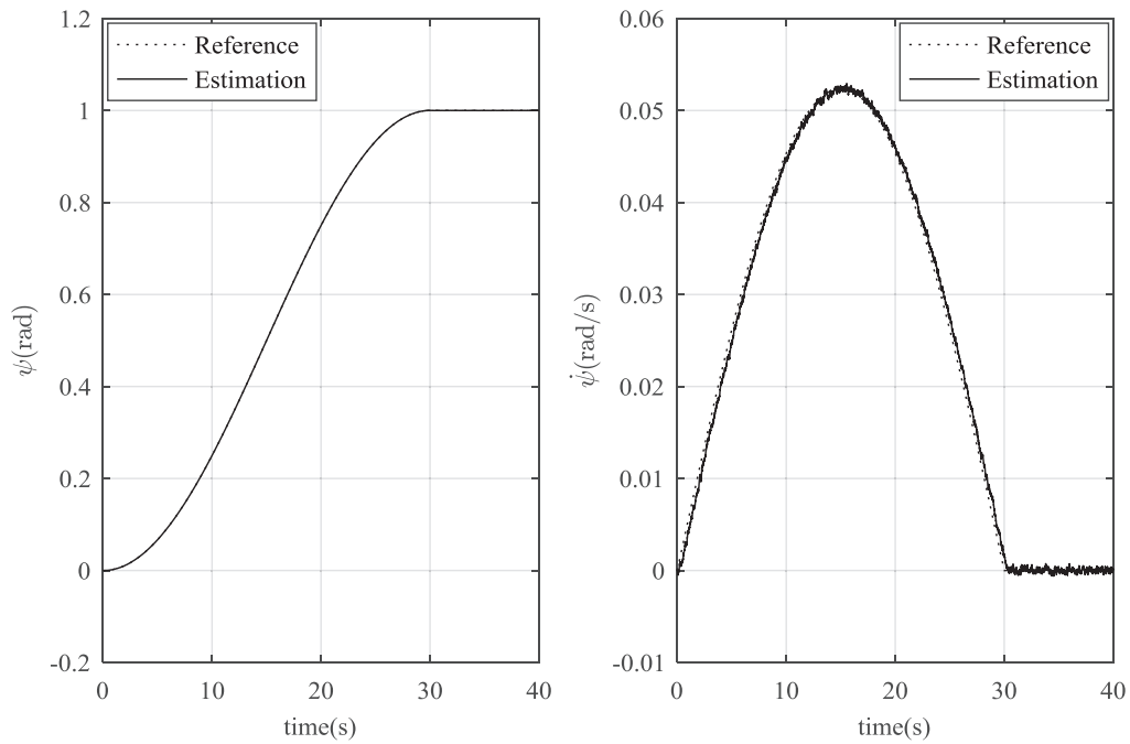
Figure 12. Simulation results of the channel \psi with measurement noise
