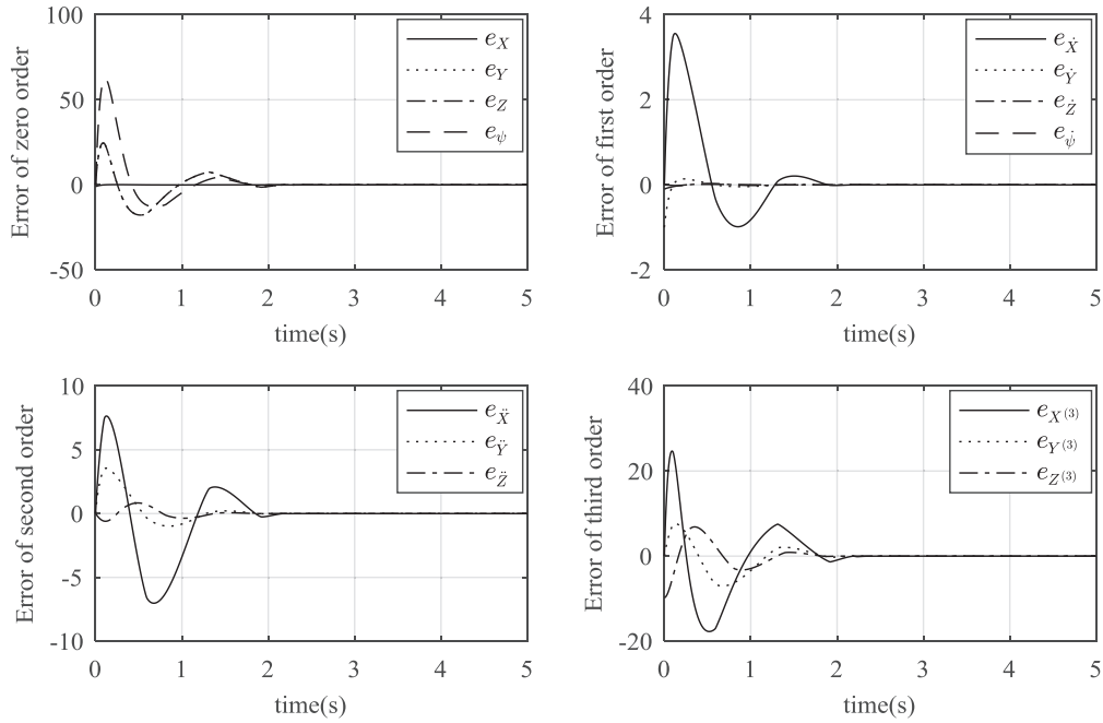
Figure 5. Estimation errors with respect to various initial differentiation errors
