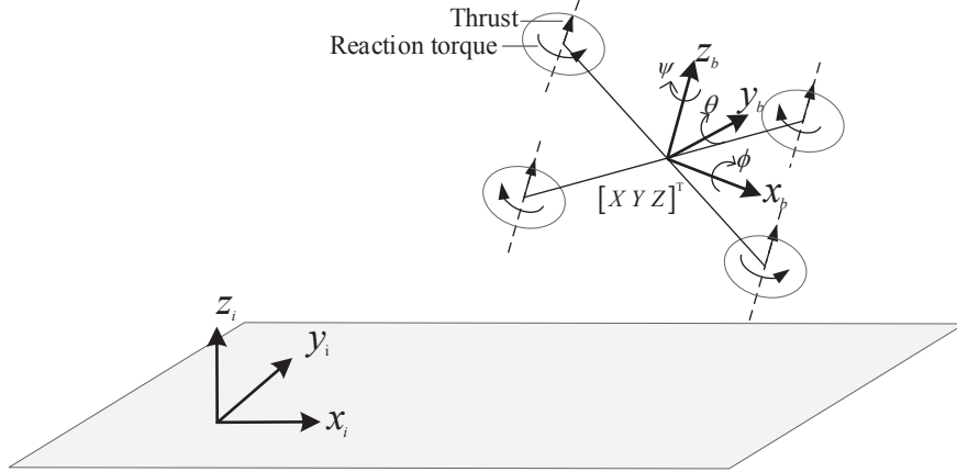
Figure 2. Quadcopter's dynamic scheme
