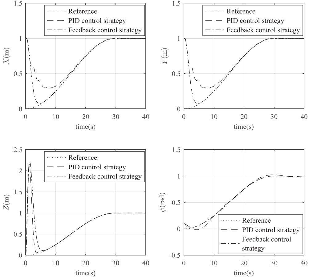
Figure 4. Control strategies' comparison
