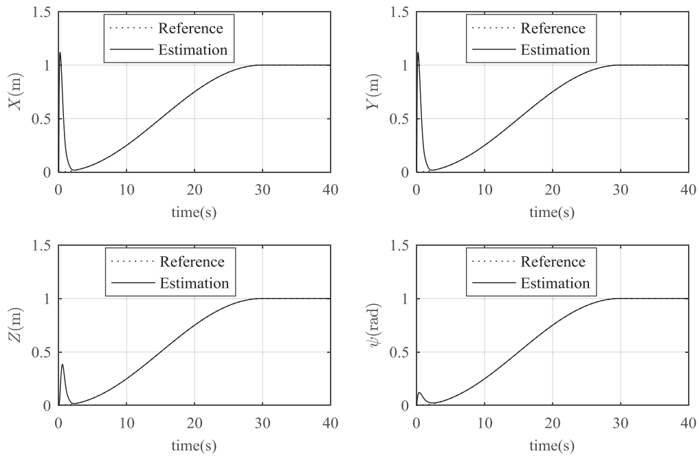
Figure 6. Output signals of the closed loop
