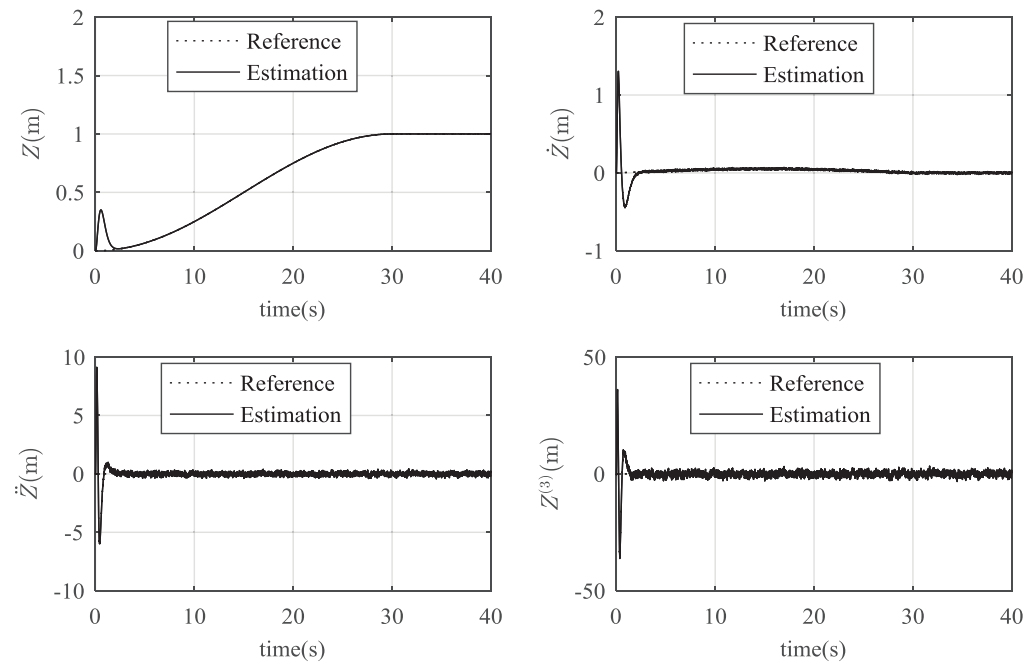
Figure 11. Simulation results of the channel Z with measurement noise
