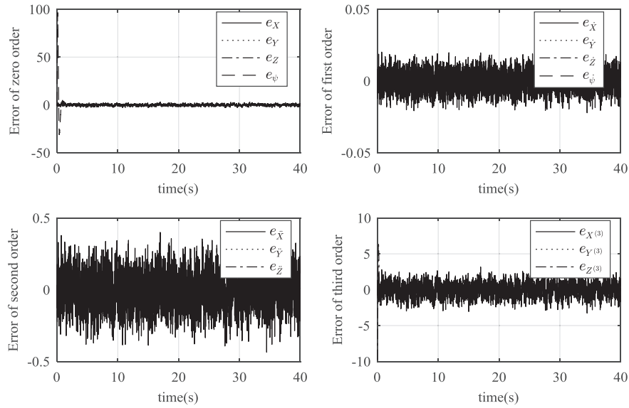
Figure 8. Errors with measurement noise
