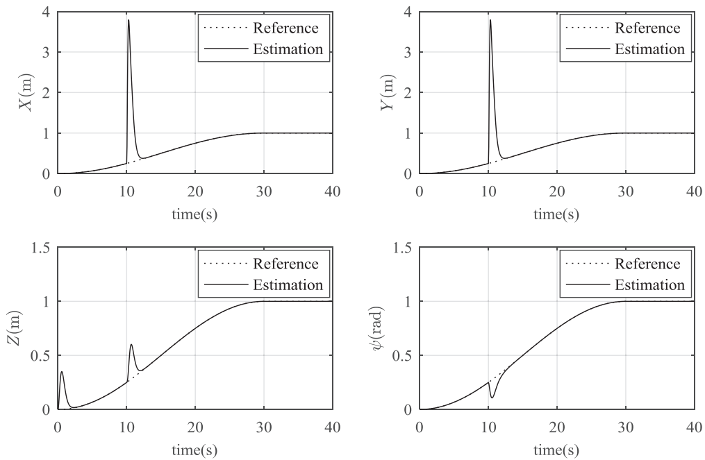
Figure 13. Simulation results in the presence of an impulsive perturbation
