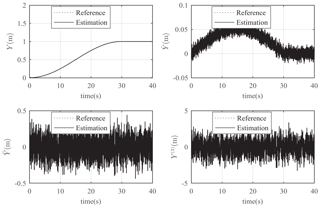
Figure 10. Simulation results of the channel Y with measurement noise
