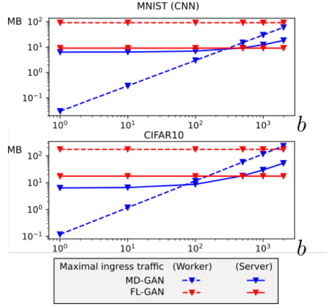
Figure 2: Maximal ingress traffic, per communication, for two types of GANs (for both MD-GAN and FL-GAN).
