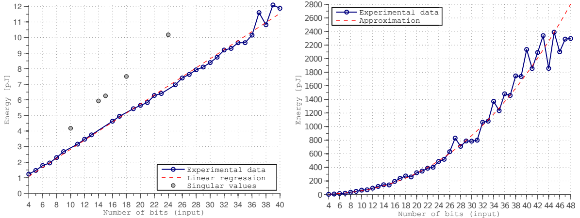
Figure 4: Energy consumption adders (left) and LUT based multipliers (right) with variable wl for Virtex-5.
