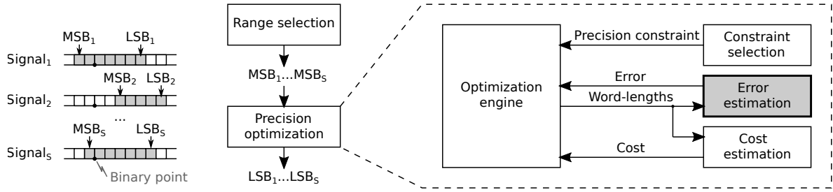
Figure 1: Basic components of a word-length optimization process
