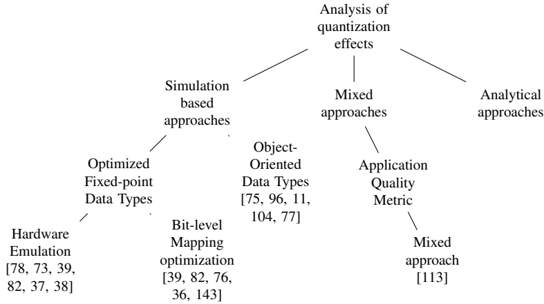
Figure 3: Classification of the different approaches to analyze the quantization noise effects
