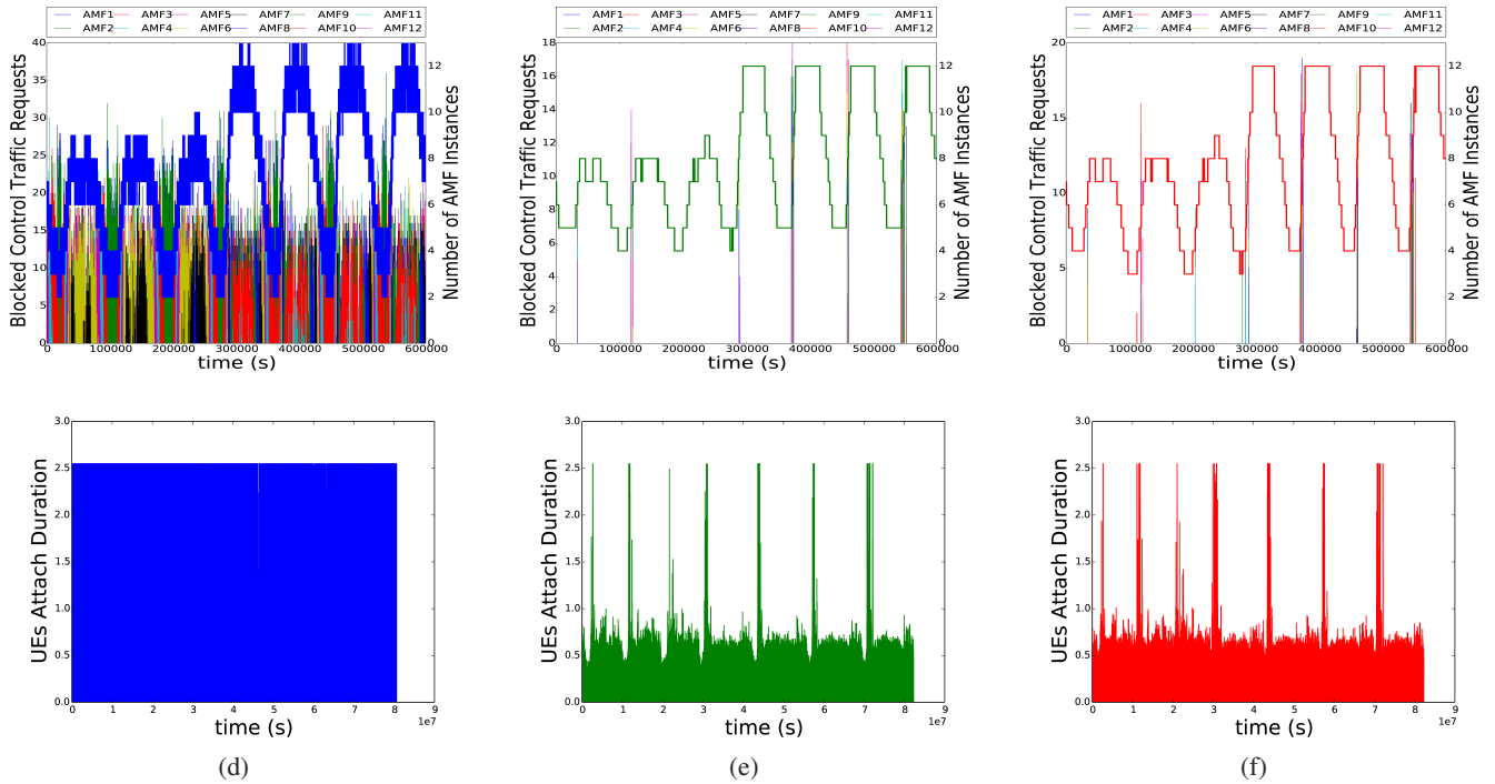
Fig. 5: AMF instances number vs Blocked traffic Requests (a) threshold-based solution (b) DNN-based solution (c) RNN-based solution compared to the evolution of the UEs attach duration (d) threshold-based solution (e) DNN-based solution (f) RNN-based solution
