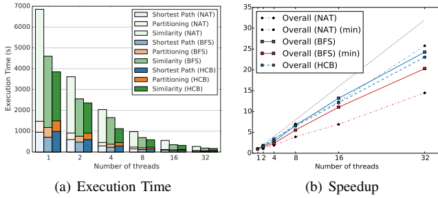
Fig. 5. Effect of data layouts to execution time and speedup in DBLP 14-17 dataset.
