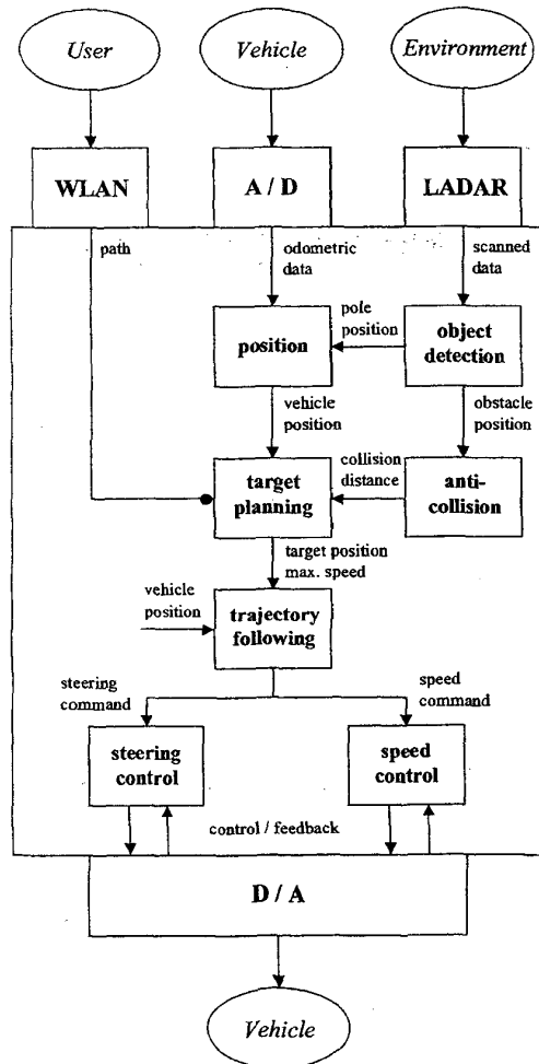
Fig. 5: Software architecture
