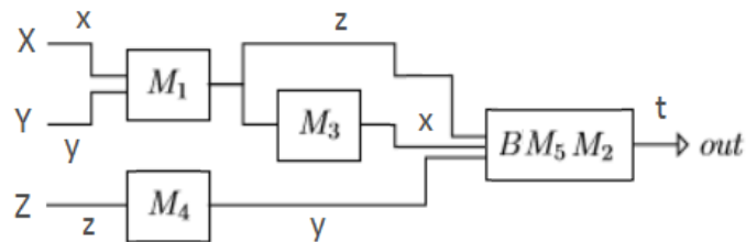
Fig.7. Reduction step 1
