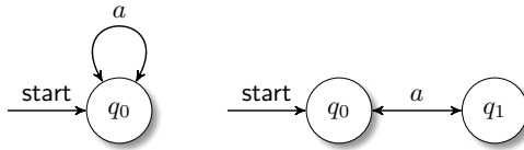
Fig. 4. Possible state graphs of unary deterministic undirected finite automata.
