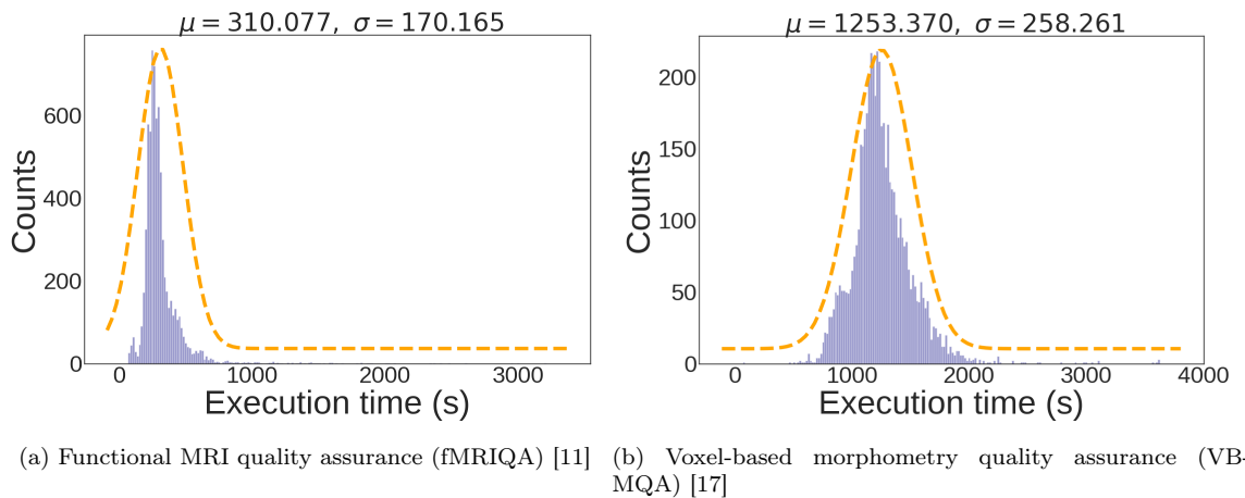
Figure 1: Traces of over 5000 runs (histograms in purple) from July 2013 to October 2016 of two neuroscience applications from the Vanderbilt’s medical imaging database [15]. We fit the data to LogNormal distributions (dotted lines in orange) with means and standard deviations shown on top.
