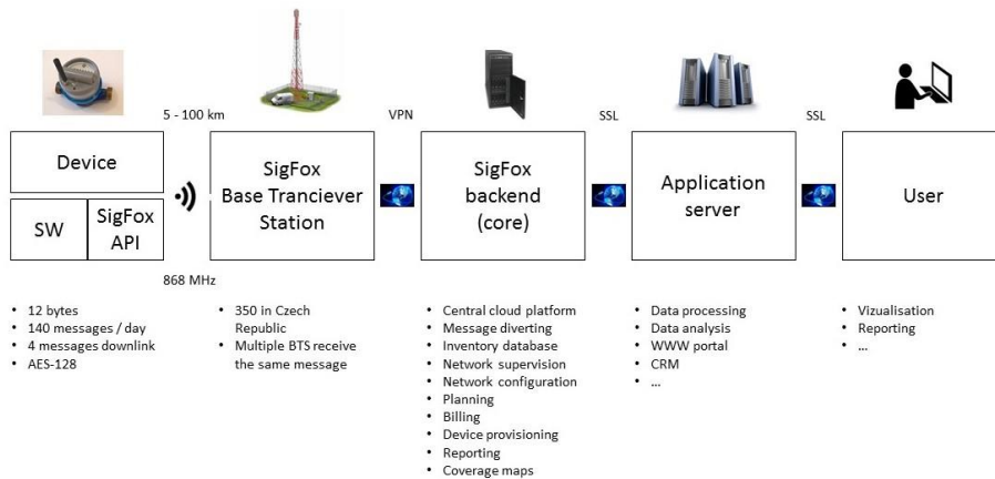
Fig. 2. Message transmission over Sigfox network
