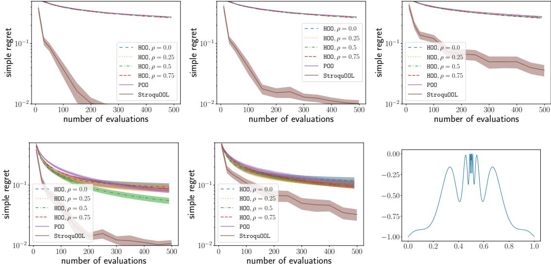
Figure 3: Bottom right: Wrapped-sine function ( d > 0 ). The true range of the noise b and the range used by H00 and P00 is \tilde{b} . Top: b = 0, \tilde{b} = 1 left — b = 0.1, \tilde{b} = 1 middle — b = \tilde{b} = 1 right. Bottom: b = \tilde{b} = 0.1 left — b = 1, \tilde{b} = 0.1 middle.
