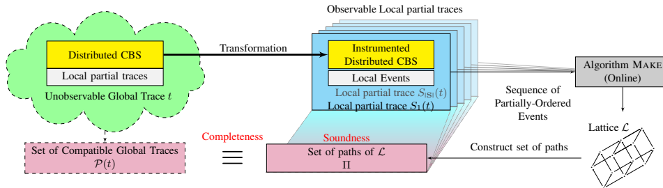
Fig. 1: Overview of the computation lattice construction
