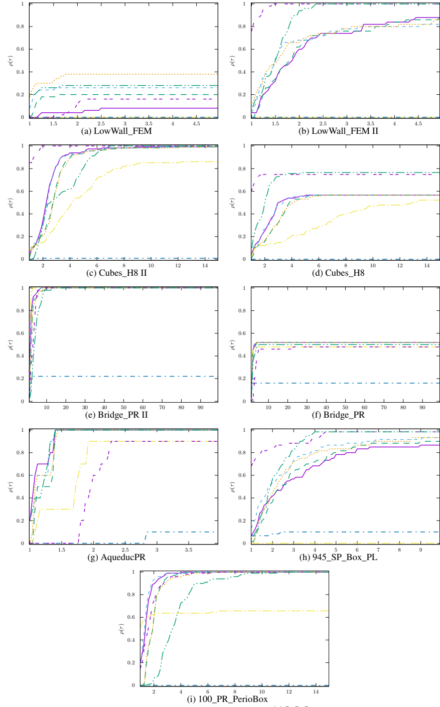
Fig. 5: Influence of the local solver in NSGS-★ algorithms.
