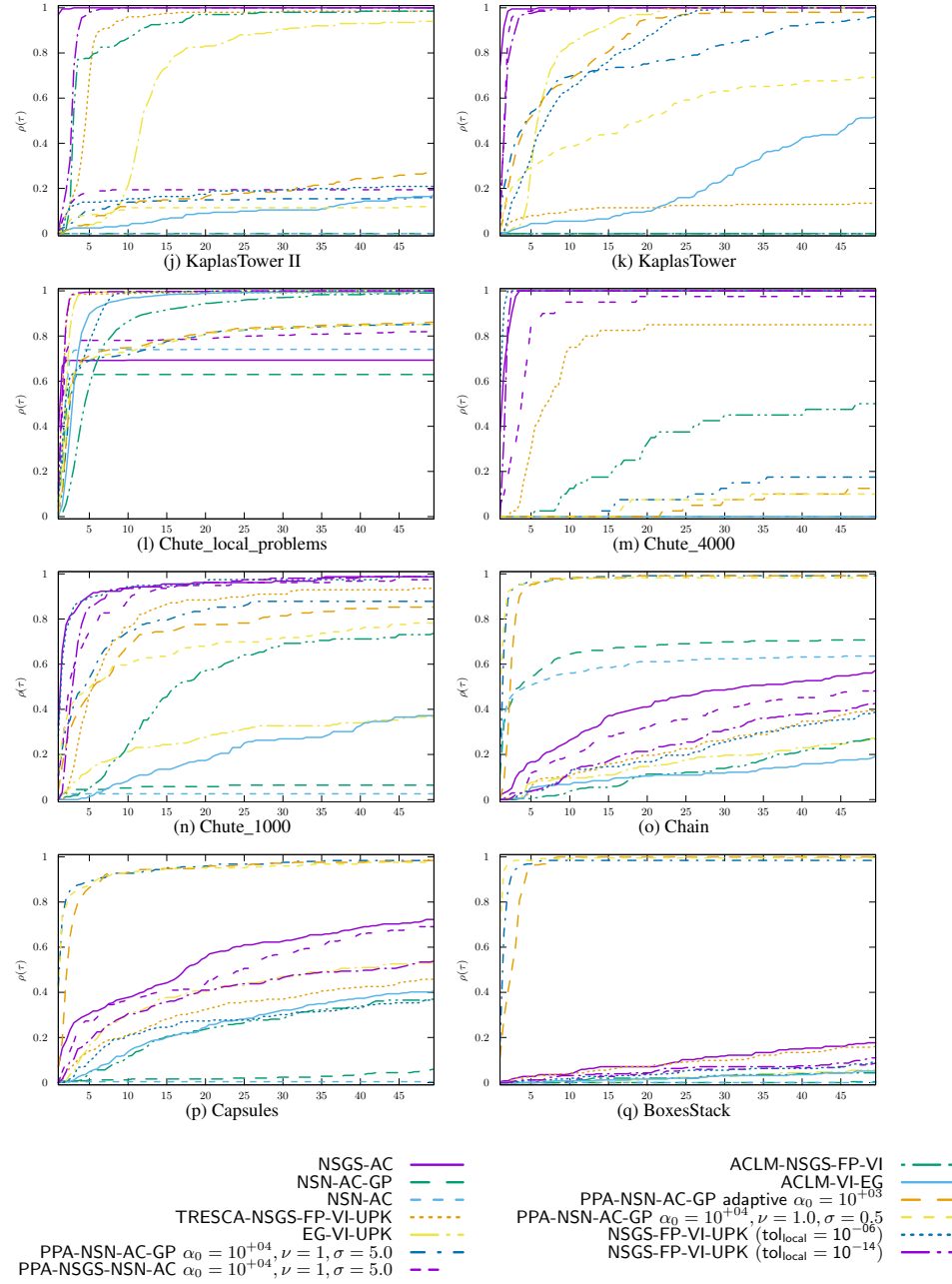
Fig. 15: Comparison of the solvers between families (continued)
