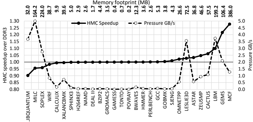
Fig. 4. HMC speedup over DDR 3 and the memory pressure (GB/s) for SPEC-CPU2006 applications.
