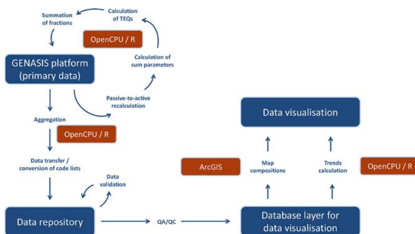
Fig. 6. Procedures and software tools employed in processing of the POPs data on their way from the primary database (GENASIS platform) to the GMP data visualisation
