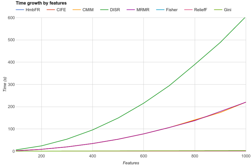
Figure 3: Scalability behavior for features growth
