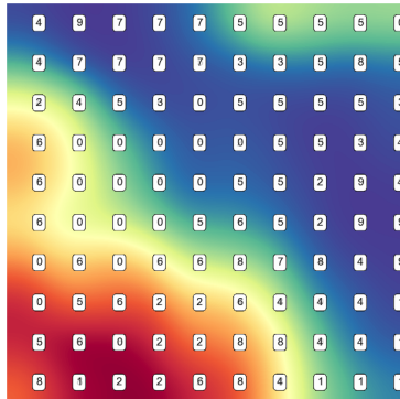
Figure 21: USPS reduced features SOM plane
