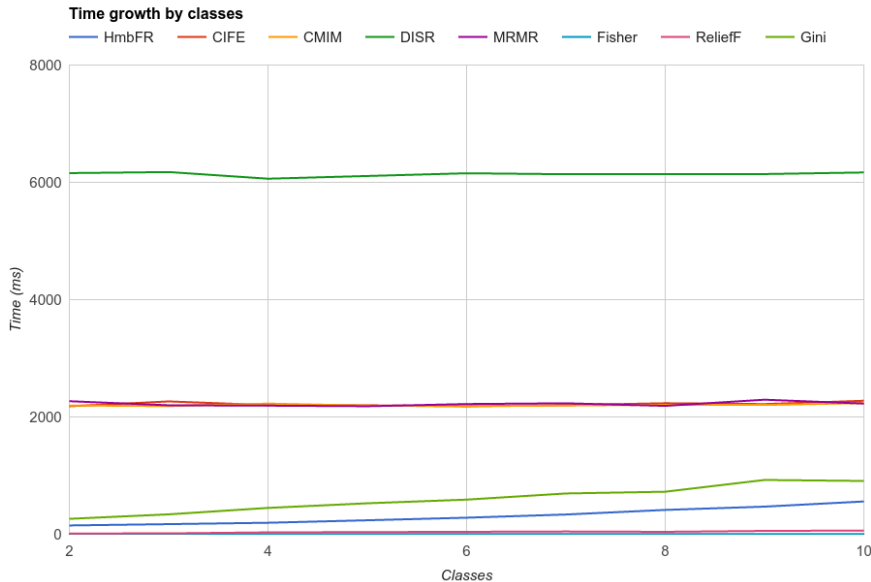
Figure 1: Scalability behavior for class growth
