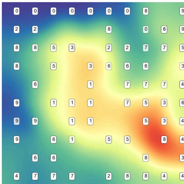
Figure 23: Warp reduced features SOM plane
