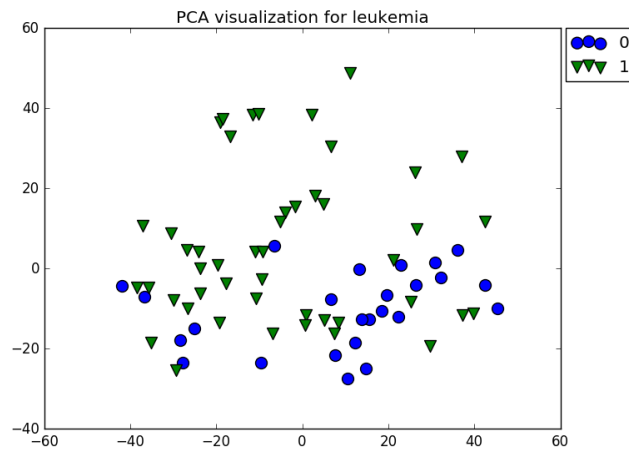
Figure 12: Leukemia Visualization
