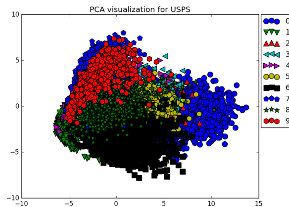
Figure 20: USPS Visualization
