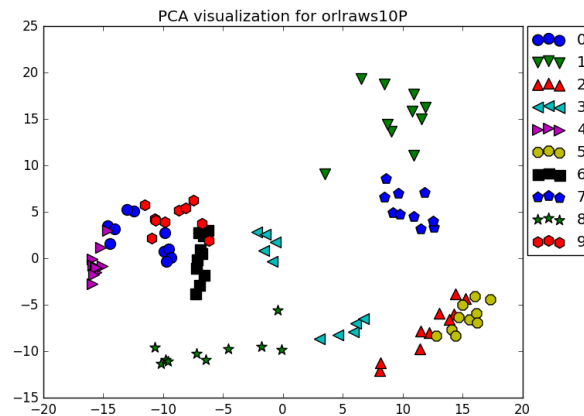
Figure 16: ORL Raws 10p Visualization
