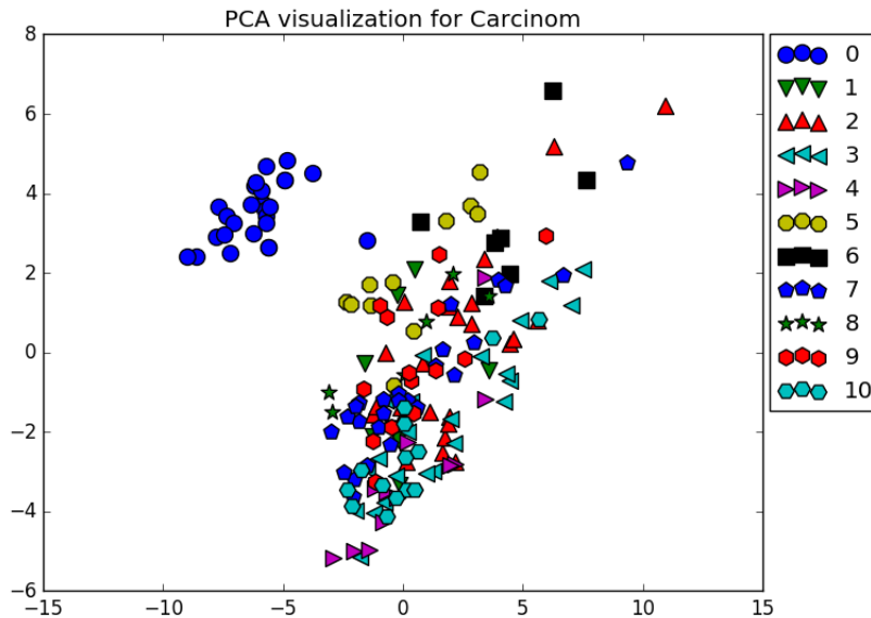
Figure 4: Carcinom Visualization
