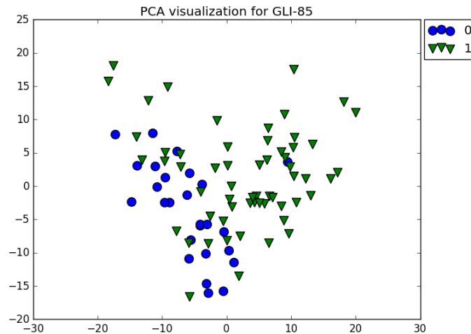
Figure 8: GLI-85 Visualization
