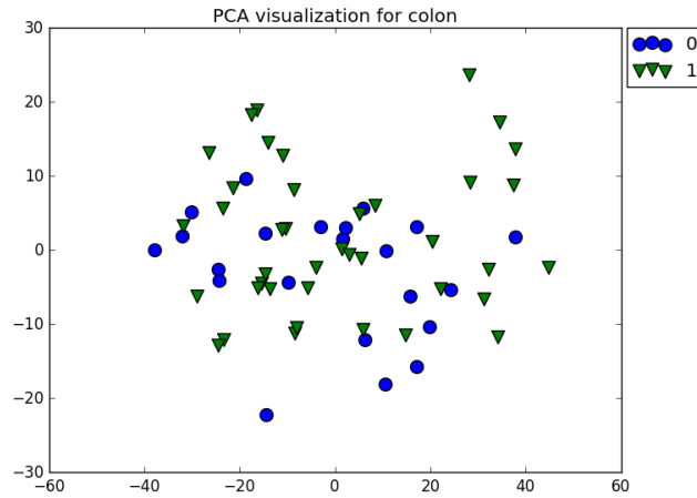
Figure 6: Colon Visualization
