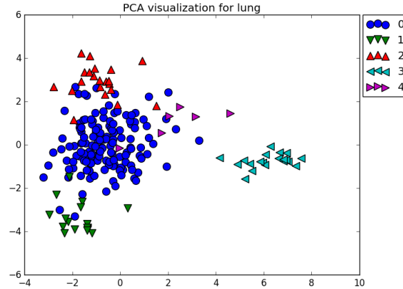
Figure 14: Lung Visualization
