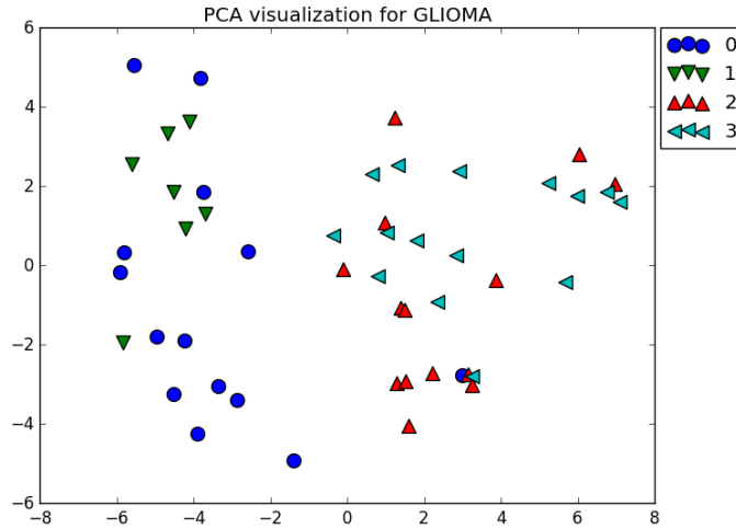
Figure 10: Glioma Visualization
