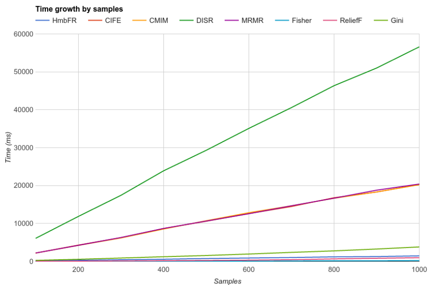
Figure 2: Scalability behavior for samples growth
