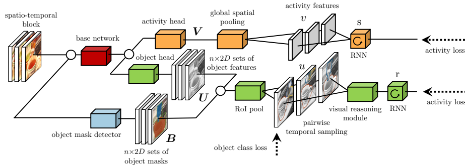
Fig. 2. A functional overview of the model. A global convolutional model extracts features and splits into two heads trained to predict, respectively activity classes and object classes. The latter are predicted by pooling over object instance masks, which are predicted by an additional convolutional model. The object instances are passed through a visual reasoning module.
