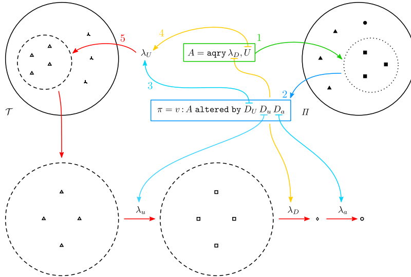
Fig. 5: Semantics of an aggregate action A given an applicable policy \pi .
