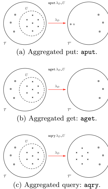
Fig. 4: Aggregation primitives.
