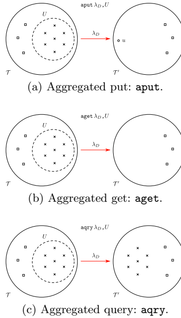
Fig. 4: Aggregation primitives.
