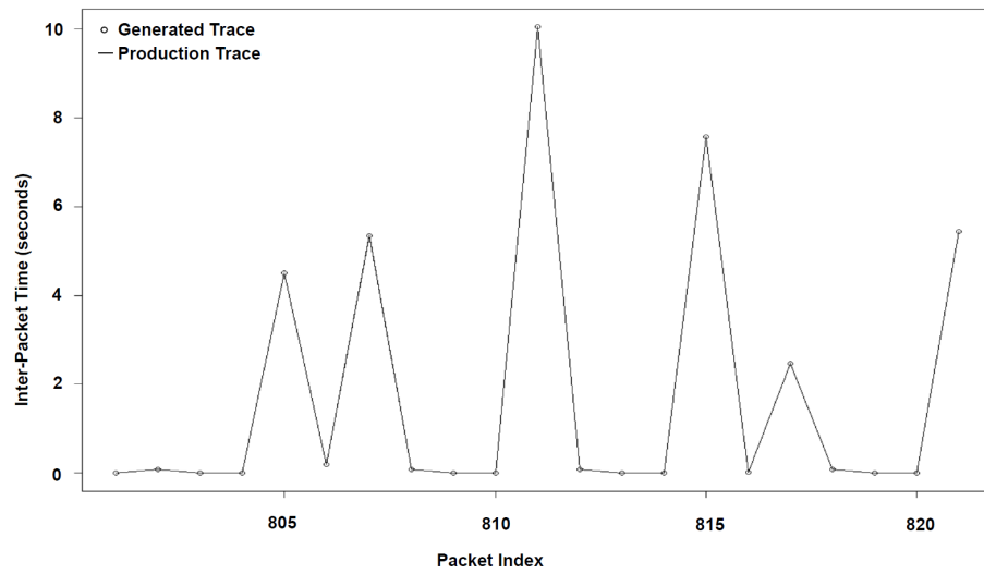
Figure 19. Detailed traffic timing pattern.
