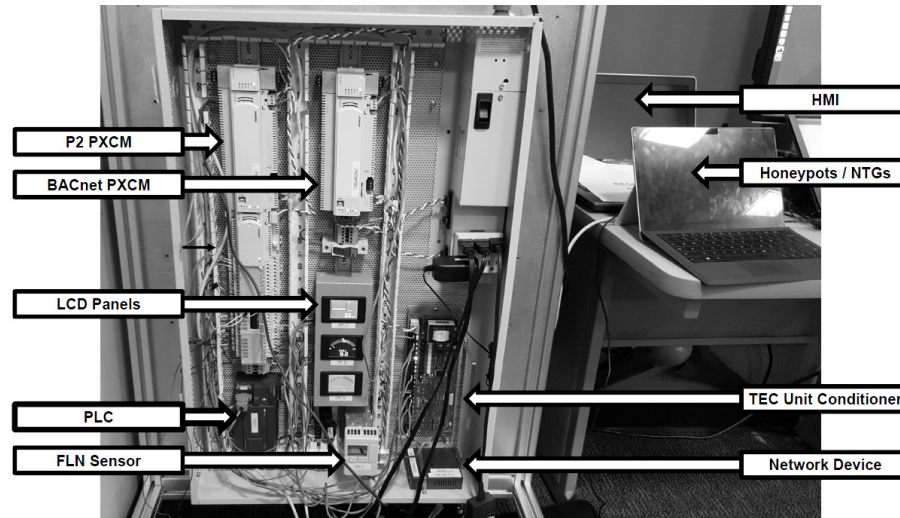
Figure 2. APOGEE platform.
