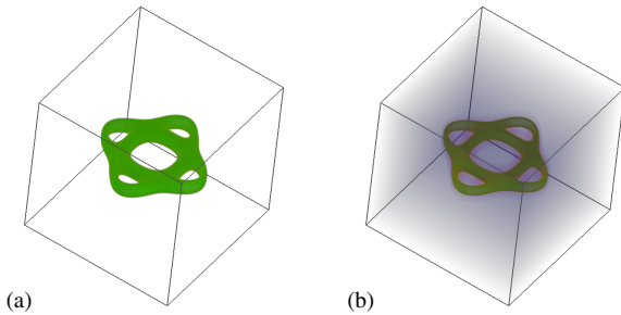
Fig. 9. DVR with transfer functions producing (a) an isosurface and (b) a foggy appearance by low but non-zero opacity values for most data values and high values for the rest.
