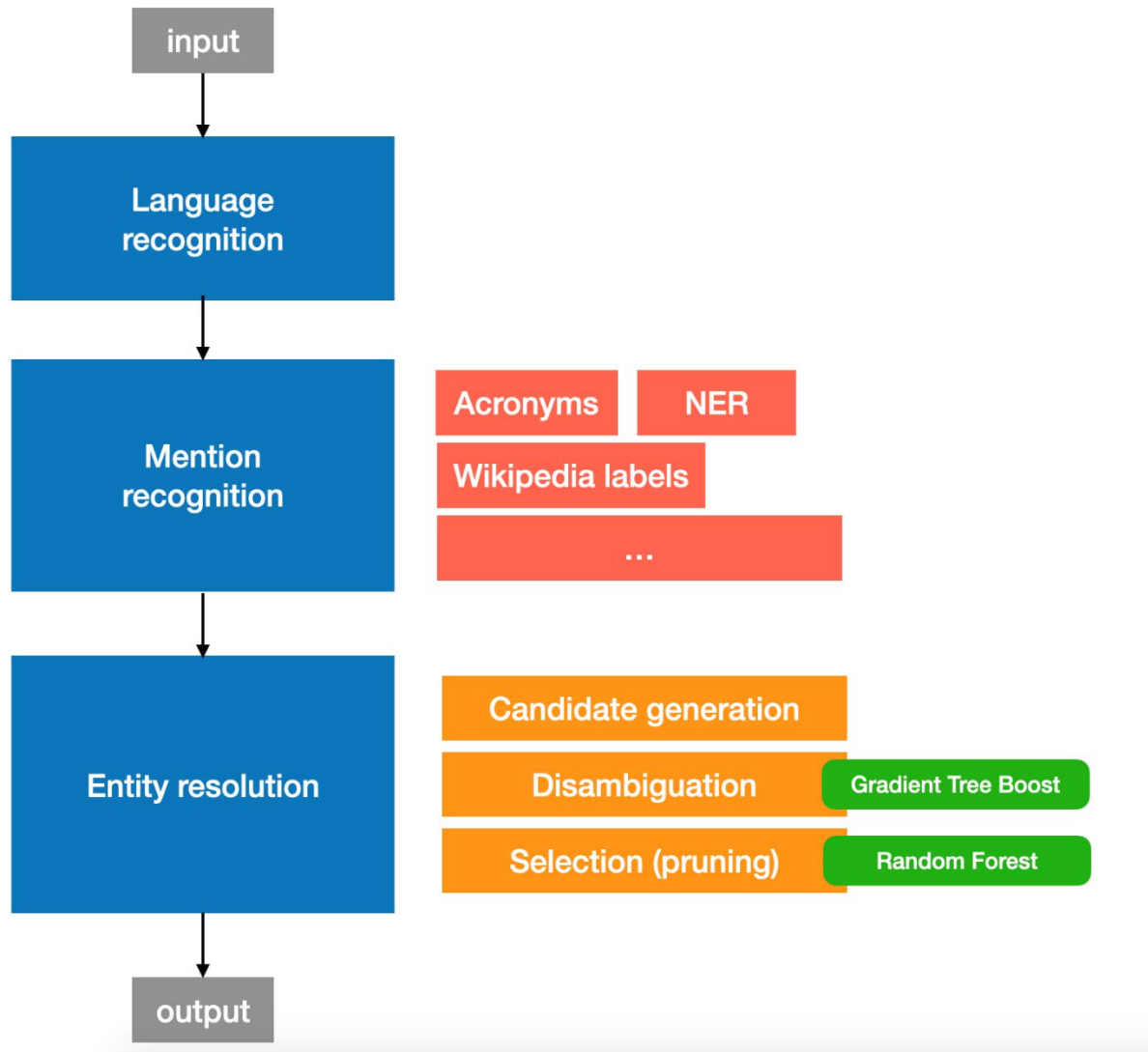
Figure 2. The data-driven architecture of entity-fishing
