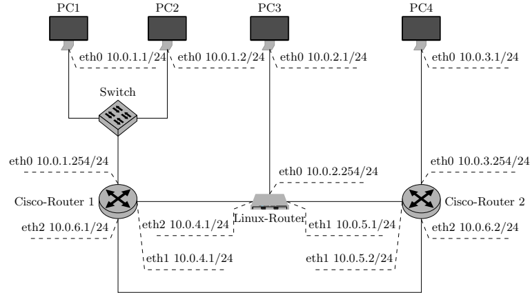
Fig. 5. Typical Infrastructure Setup within the iLab Course
