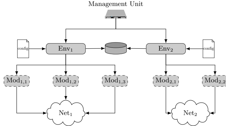
Fig. 3. Information Collector Component of INSALATA
