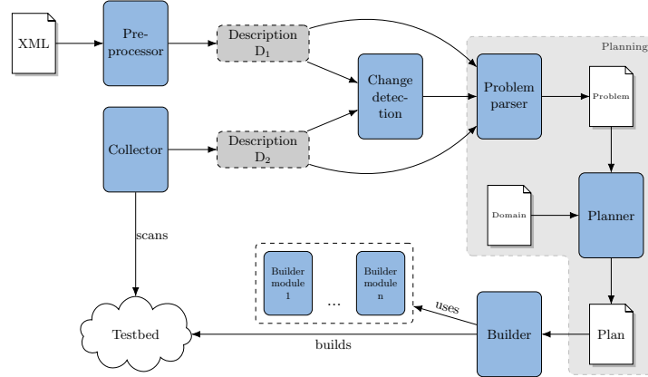
Fig. 4. Execution Flow of INSALATA's Deployment Component
