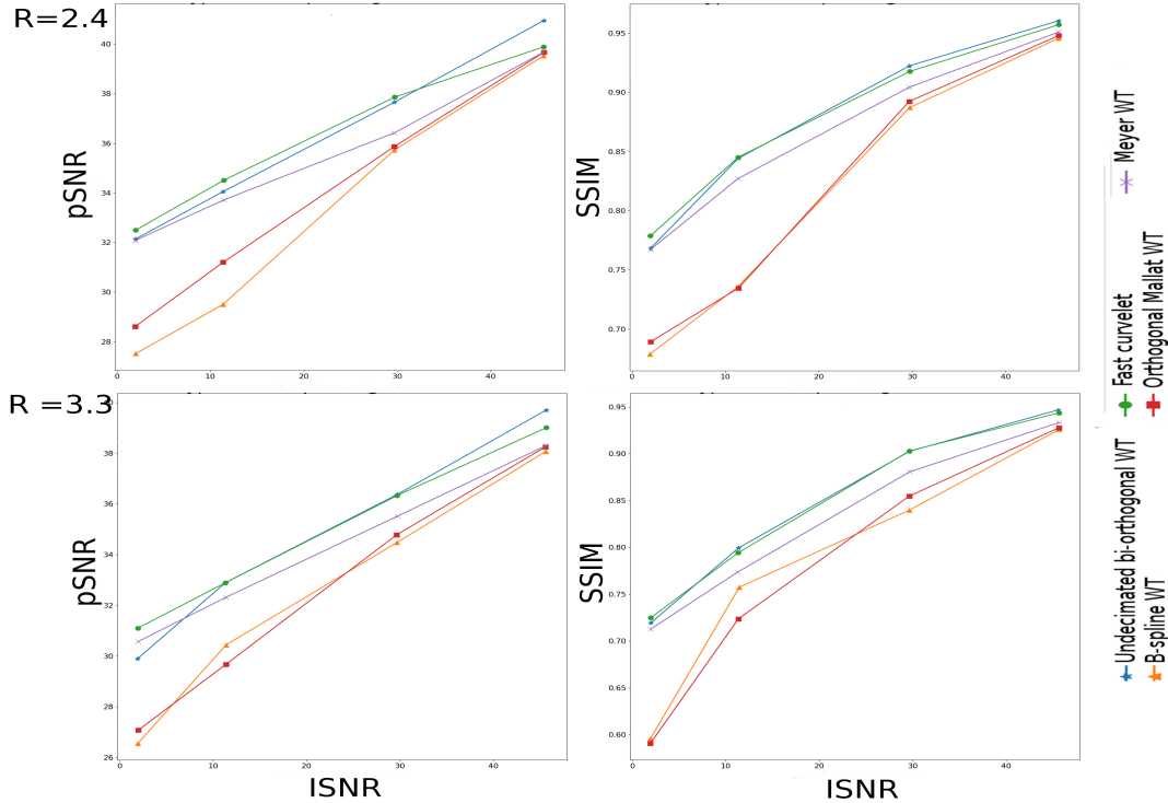
Fig. 3. pSNR (left) and SSIM (right) scores after CS-PI MR image reconstruction from retrospectively under-sampled k -space data using Sparkling under-sampling schemes (top: R = 2.4 , bottom: R = 3.3 ). Each line codes for a specific multiscale decomposition, see the legend within each panel.
