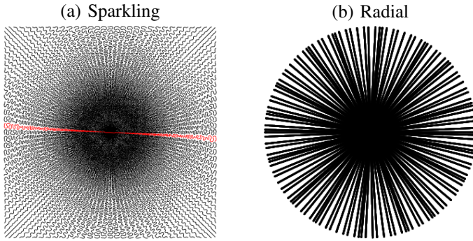
Fig. 1. Non-Cartesian multi-shot under-sampling schemes for R = 2.4 i.e., 40 % of full- k -space measurements.
