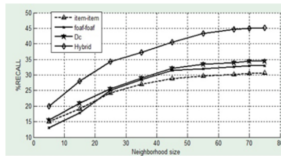
Fig. 4. Recall rate
