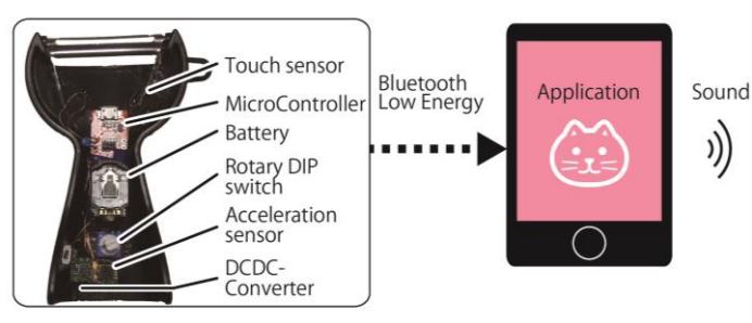
Fig. 2. System Configuration
