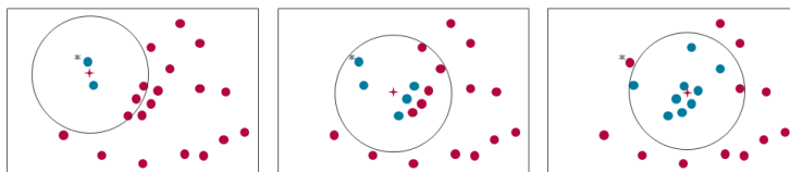
Fig. 2: Illustration of the spatial density-based clustering
