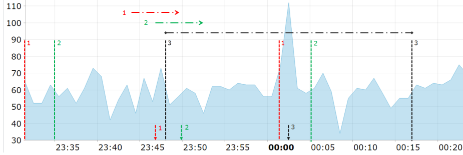
Fig. 3: The intensity-based fragmentation of the timeline (temporal clustering)
