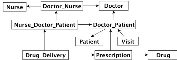
Fig. 7. A small part of the ASIS-IS schema of the hospital
