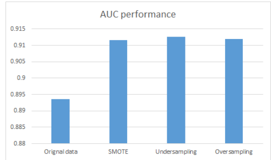
Fig. 7. Performance in term of AUC values using preferential attachment and TF-IDF values.
